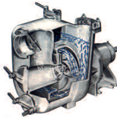
Impeller: Open impeller handling large diameter spherical solids
