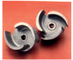
Impeller: Open impeller handling large diameter spherical solids
